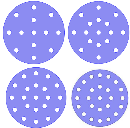
Fig. 6 Number of HTF tubes taken for optimization
