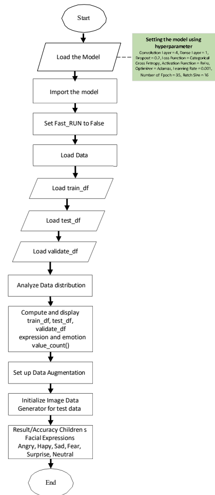
Fig. 1 Flowchart of Classification System in CNN
