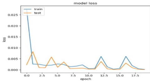
Fig. 5 Loss for Dataset-A
